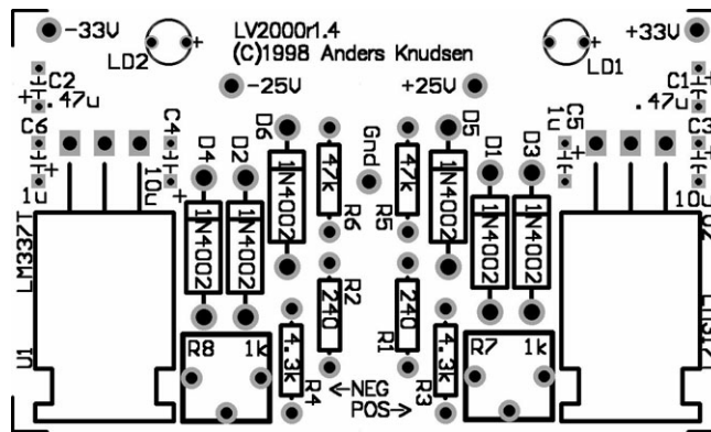
LV2000 PCB Silkscreen
