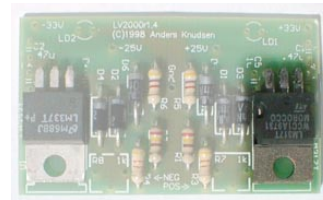
LM317T (+)
