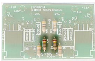
R1 & R2 – 240 ohm (Red/Yellow/Brown)
