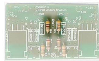
R5 & R6 – 4.7k (Yellow/Purple/Red)
