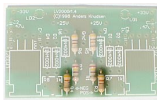
R3 & R4 – 4.3k (Yellow/Orange/Red)
